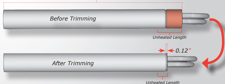
Heater size at Maximum Length Tolerance ( ALL cavity must be trimmed). 31.86"
